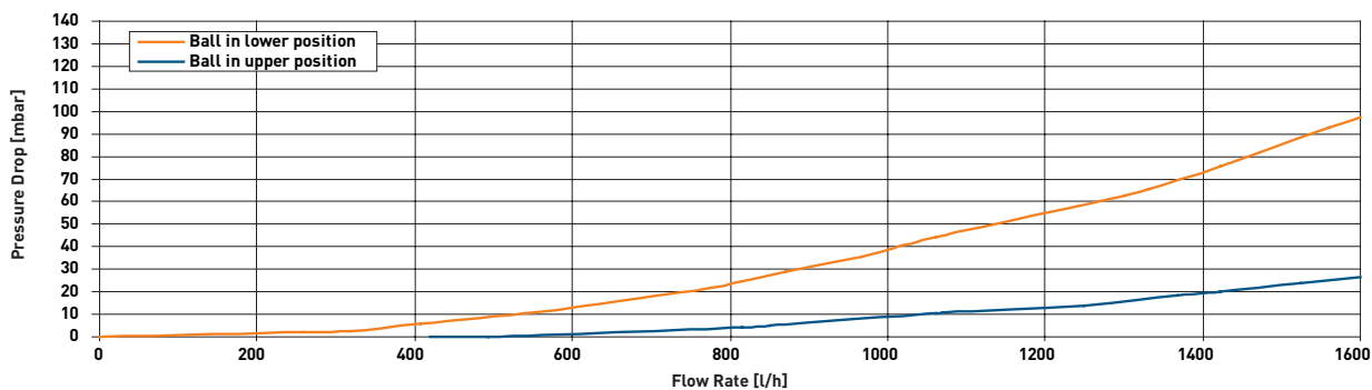
Flow curve
