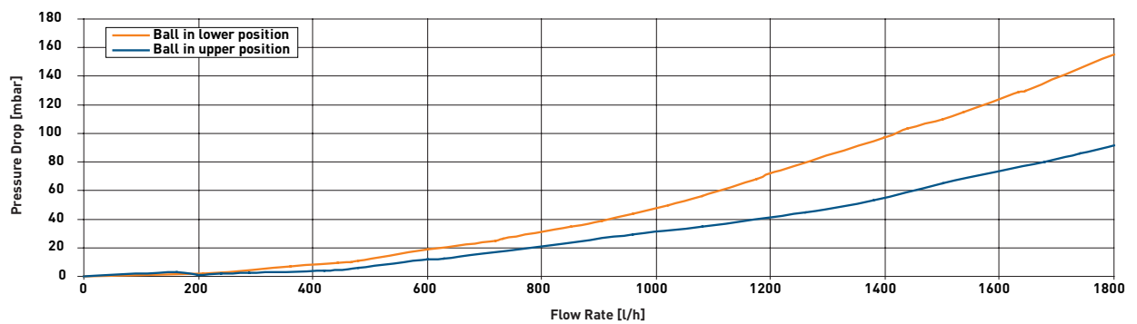
Flow curve
